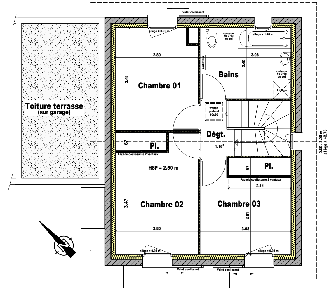
Lot -05- (P.S.L.A.) Plan: Etage
